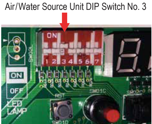
Figure 3: Location and Setting of Outdoor Unit DIP Switch 3.
